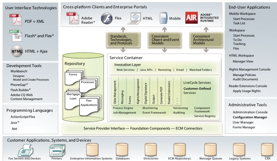
The LiveCycle ES3 architecture
