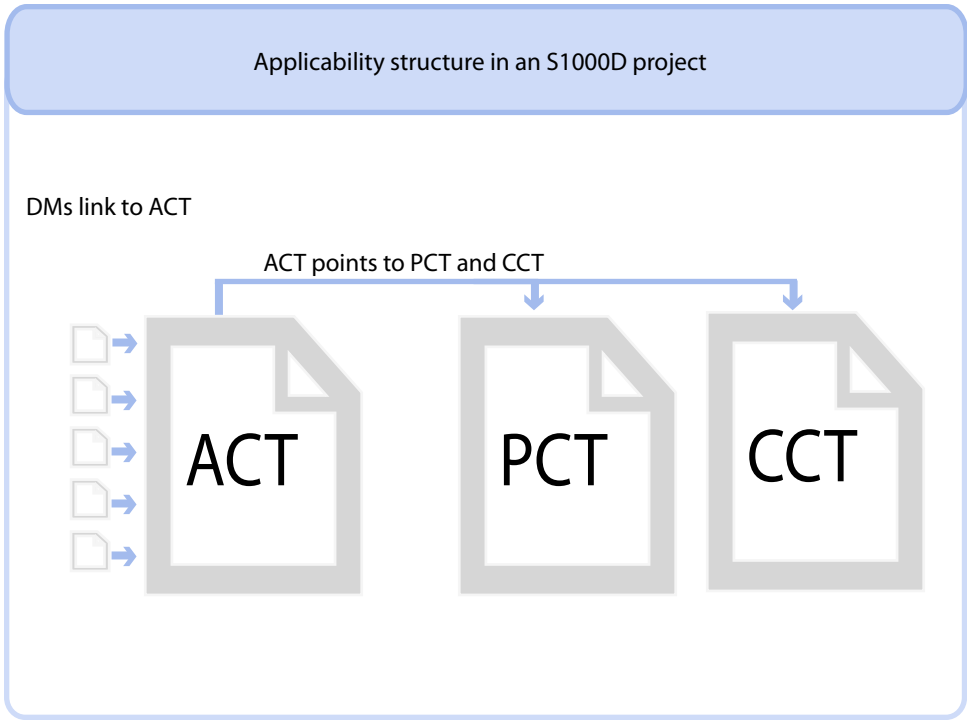
Linking of the Applicability modules of S1000D
