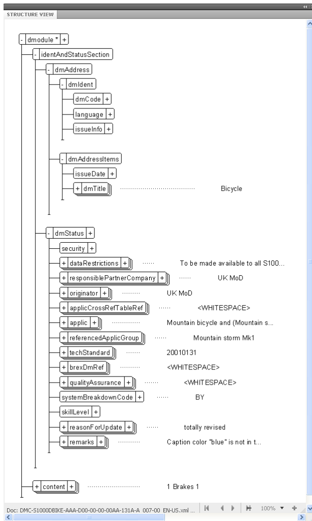
Structure of the idstatus section
