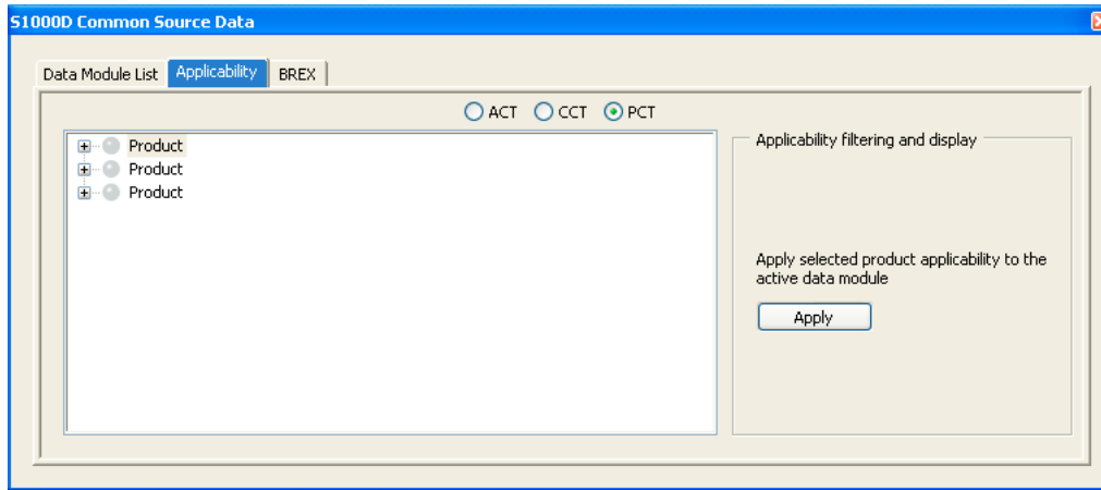
PCT part of S1000D Common Source Data dialog's Applicability tab
