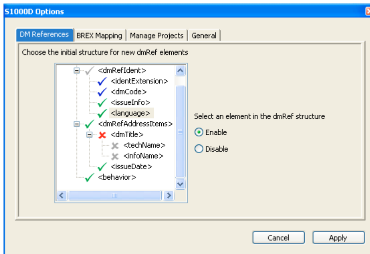
S1000D Options - the DM references tab
