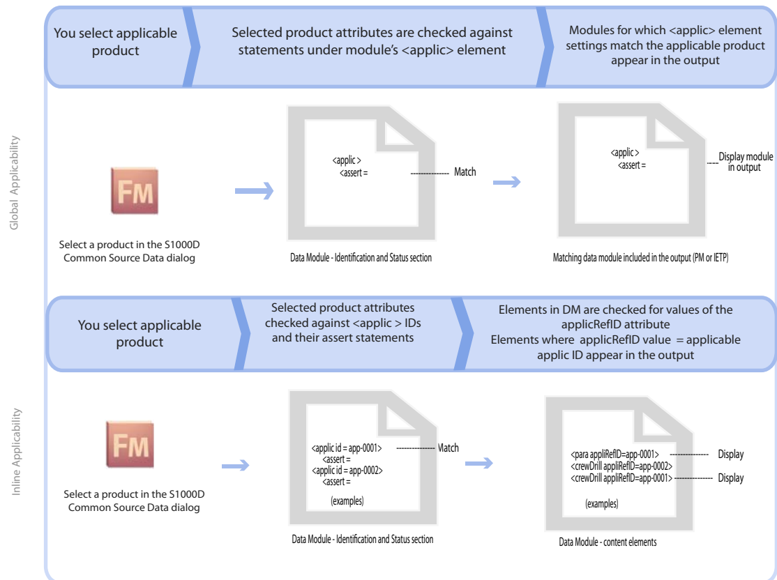
Overview of global and inline applicability processes
