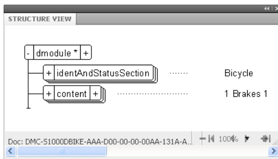
Structure of a data module
