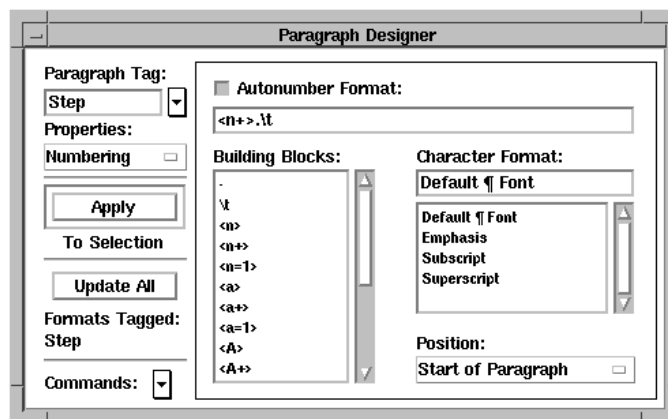
Figure 2-12 Paragraph Designer
