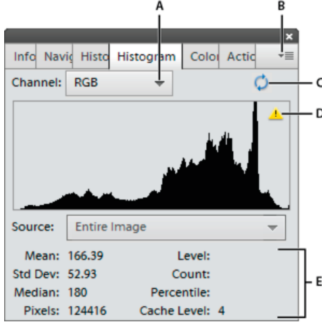
Histogram paneli
