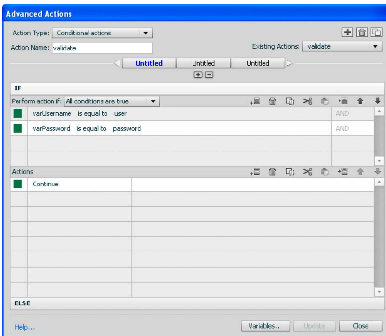
IF condition in the 'validate' advanced action
