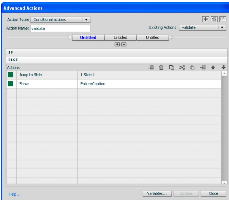
ELSE condition in the 'validate' advanced action
