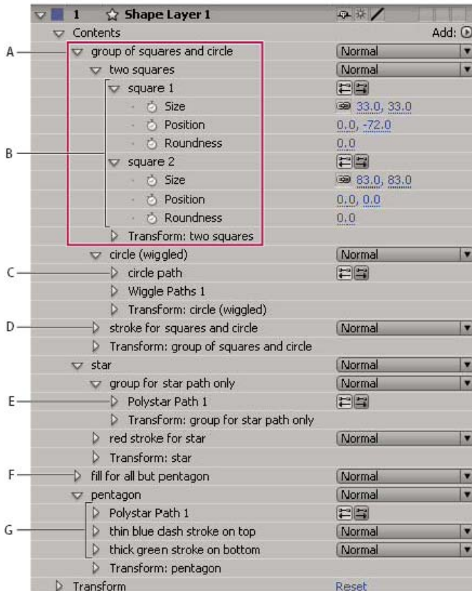
A. Two shapes in a group B. Two paths in a compound shape C. Circle path with Wiggle Paths applied D. One stroke applied to all paths above it E. Star path in a group by itself F. One fill applied to all paths above it G. One path with two strokes
