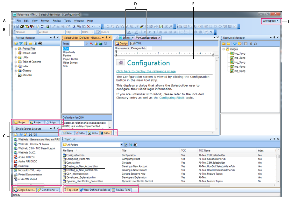
RoboHelp workspace
